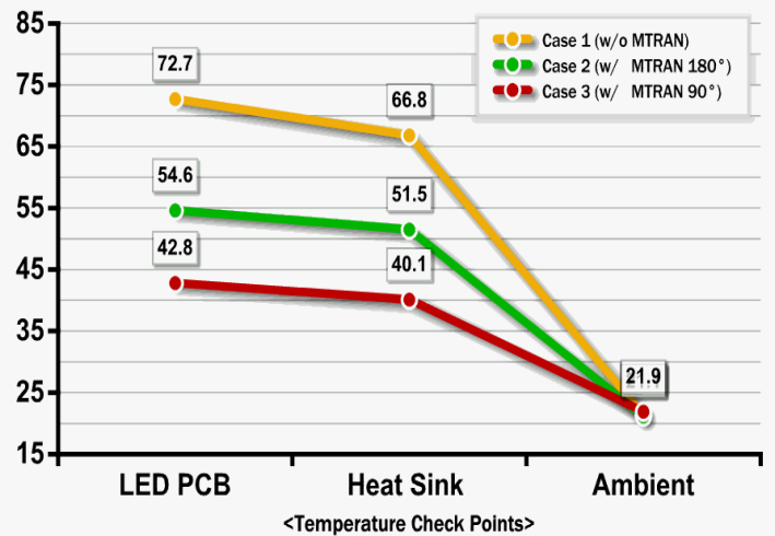
5W LED(The Diamond Dragon) Thermal Test Results
